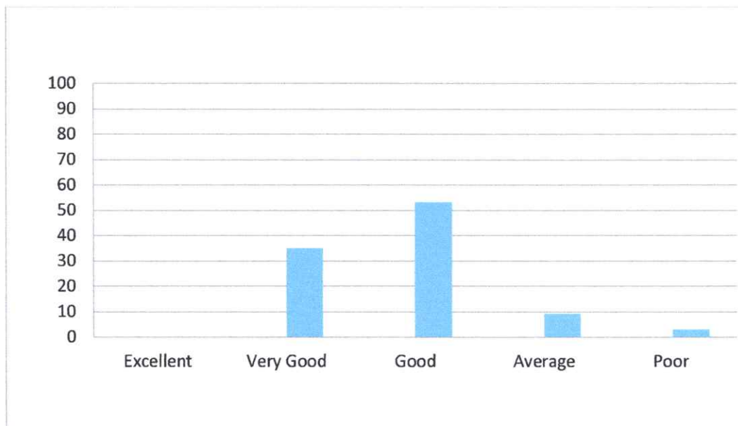
Graph 7. How do you rate the domain knowledge used for desiring the experiments in terms of the suitability of the Tools to the domain?
