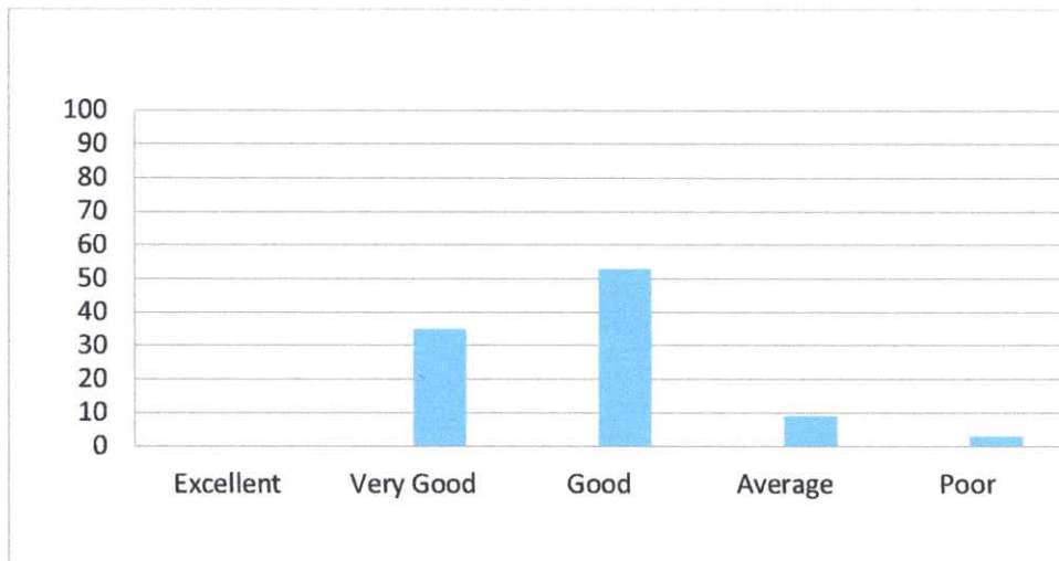
Graph 1: How do you rate the program that your ward undergoing in terms of the load of the courses in different years / semesters?
