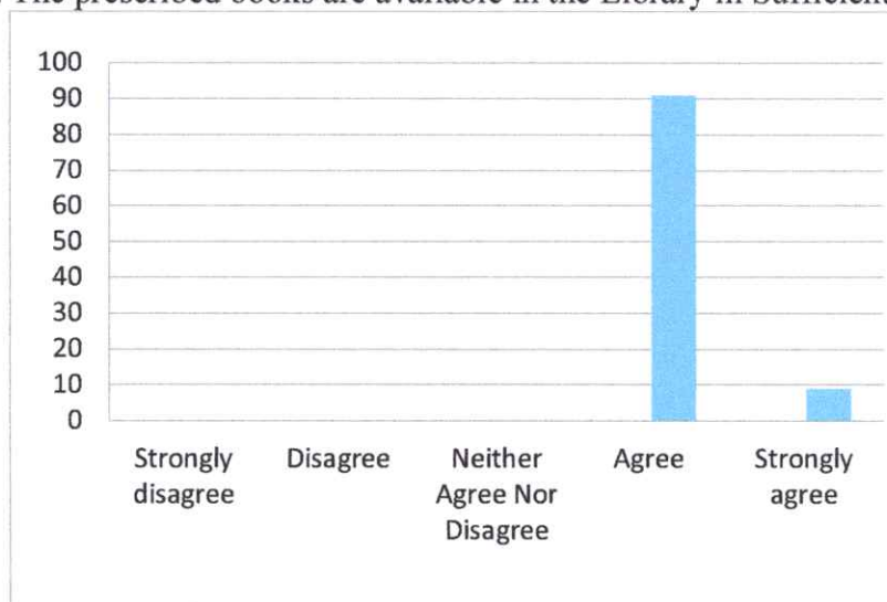
Graph 8: The prescribed books are available in the Library in Sufficient numbers'
