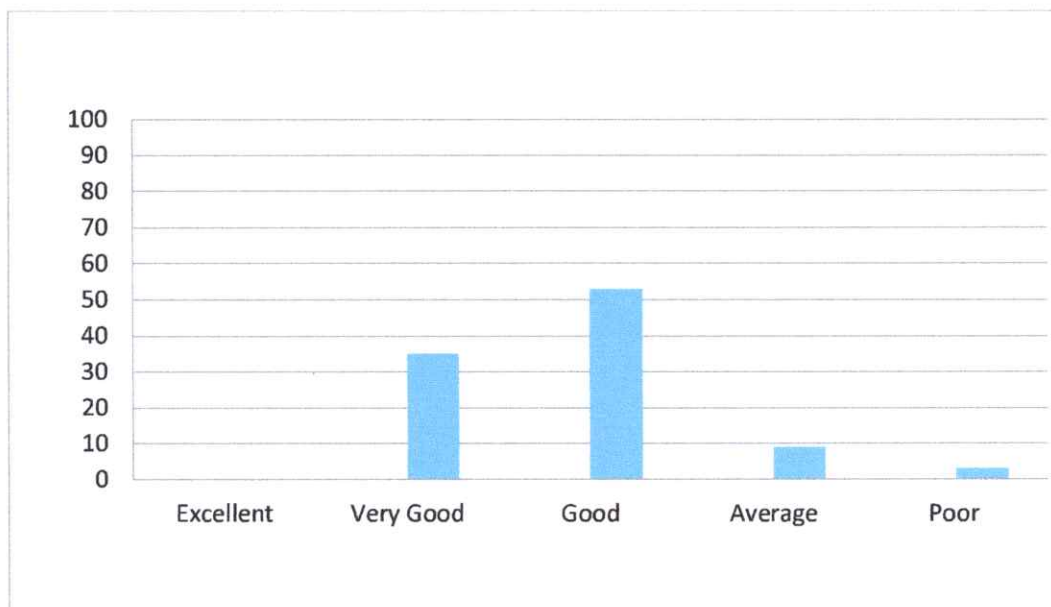
Graph I: How do you rate relevance of the courses in relation to the program?
