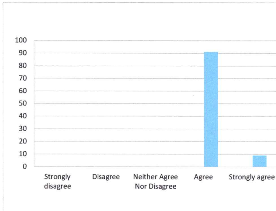
Graph 2: The objectives of the syllabi are well defined.
